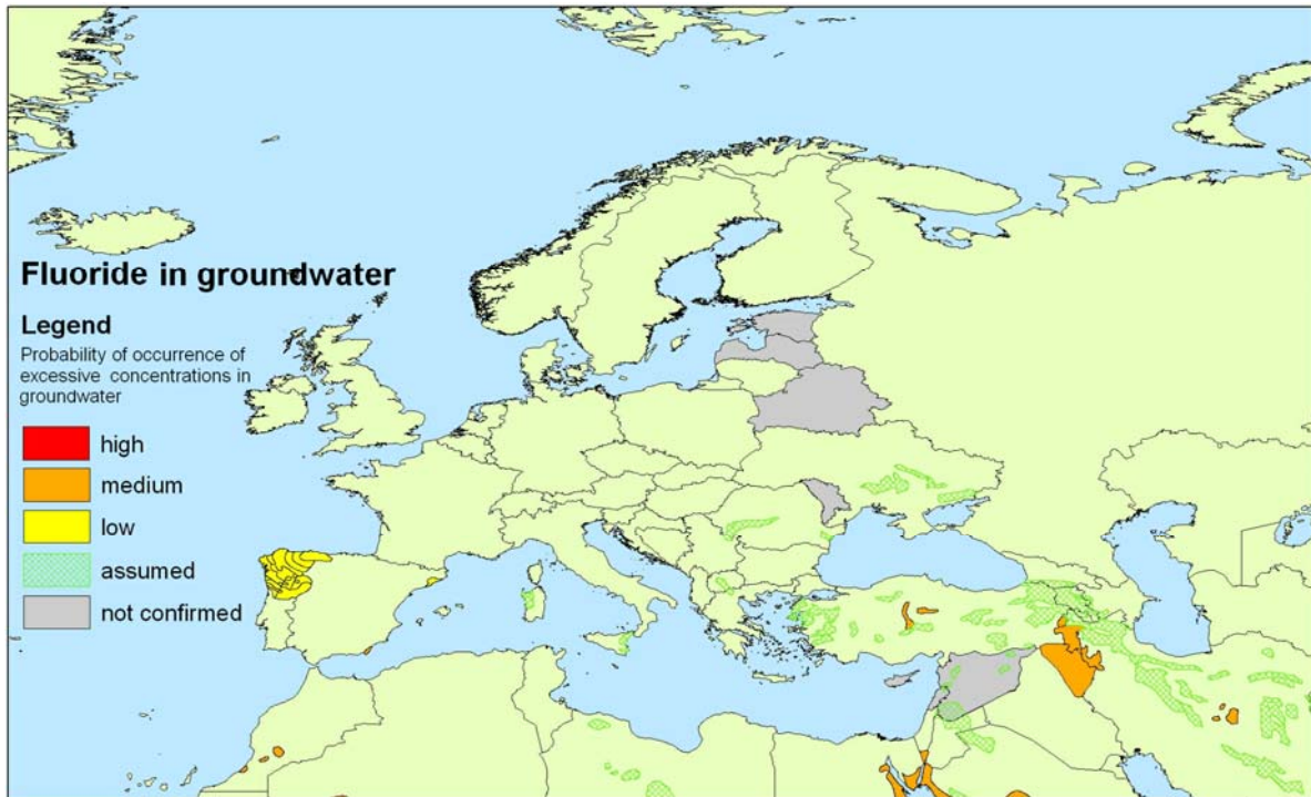
Figure 3 Fluoride in groundwater in Europe
